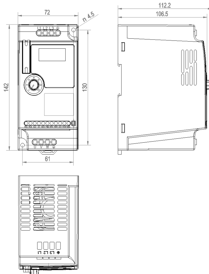
Dimensional drawing A550 Plus - 1,5kW 4T0015
