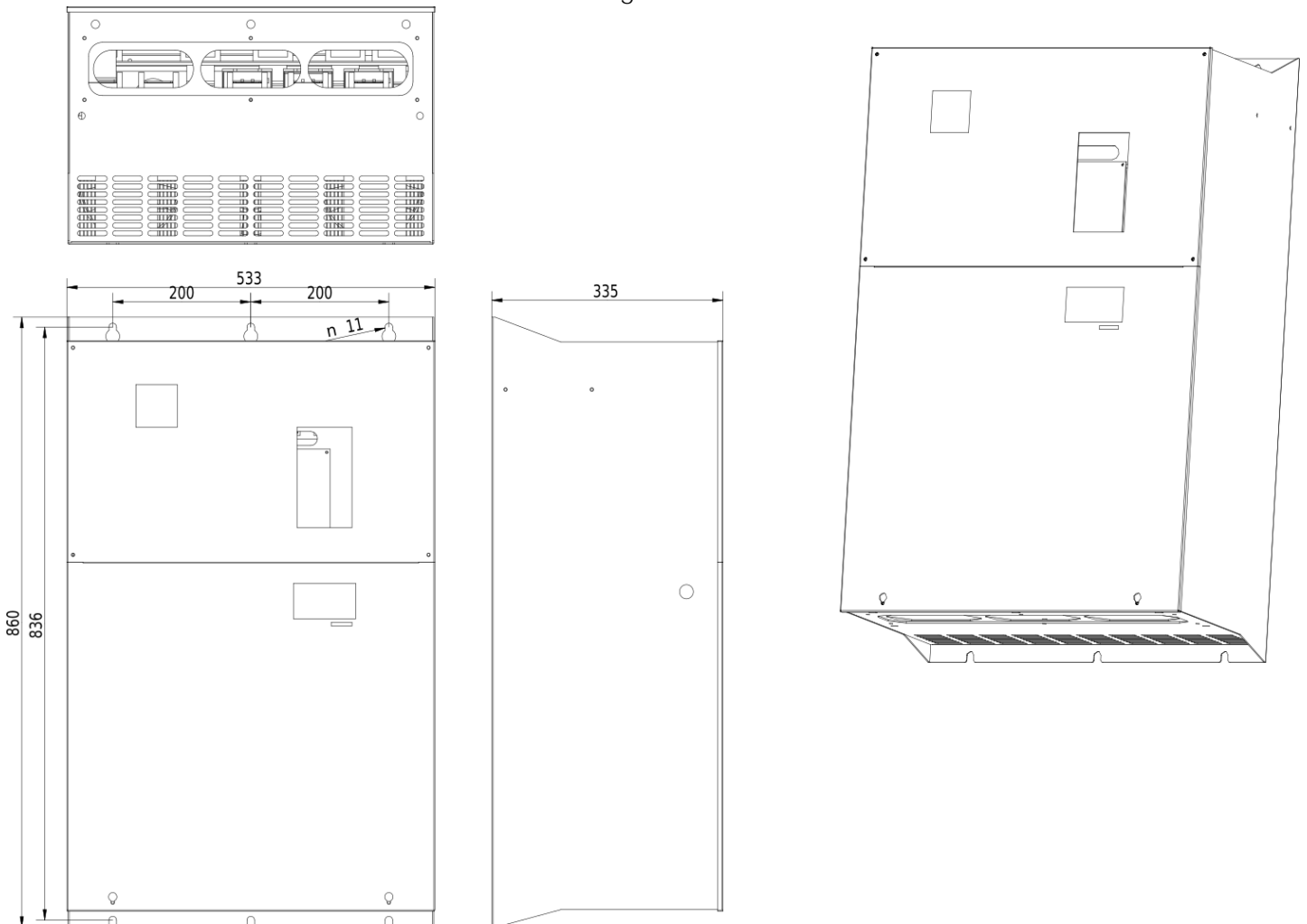
Dimensional drawing V810 - 220kW 4T2200
